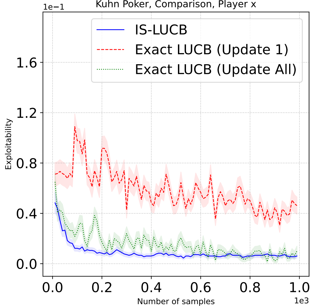
Kuhn Poker, Comparison, Player x
